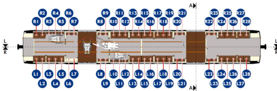
PTOS car saloon interior seat plan
