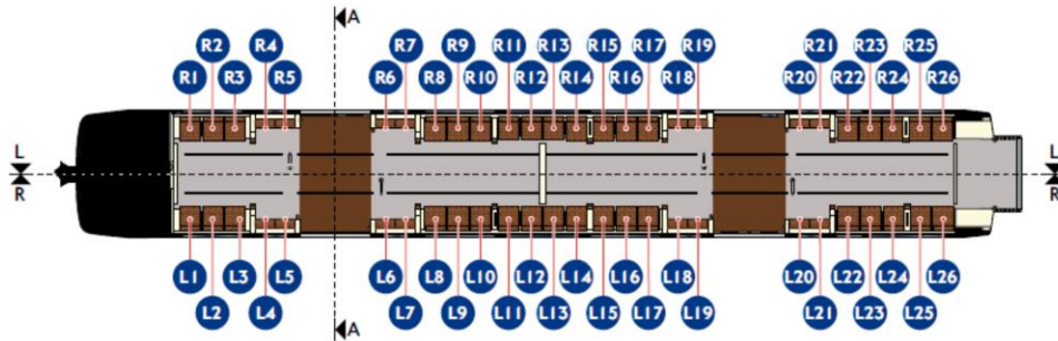
DMOS car saloon interior seat plan
