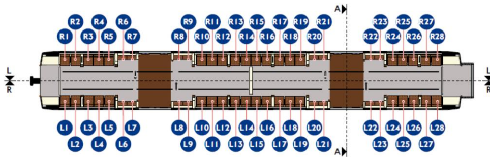
MOS car saloon interior seat plan
