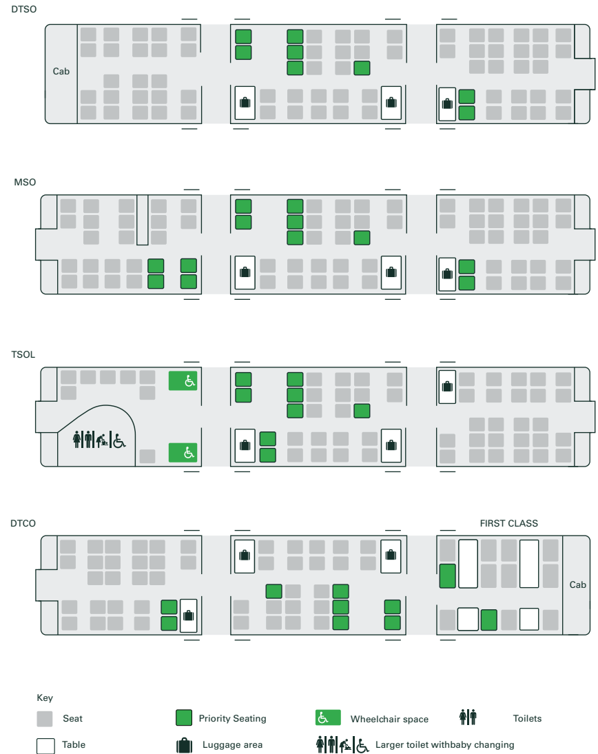
Class 769 Flex seating plan
