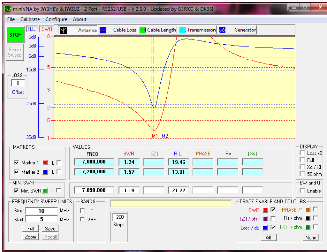
MINIVNA Chart for 40M (7.00, 1.35, 7.125 1.28, 7.2, 1.18)
