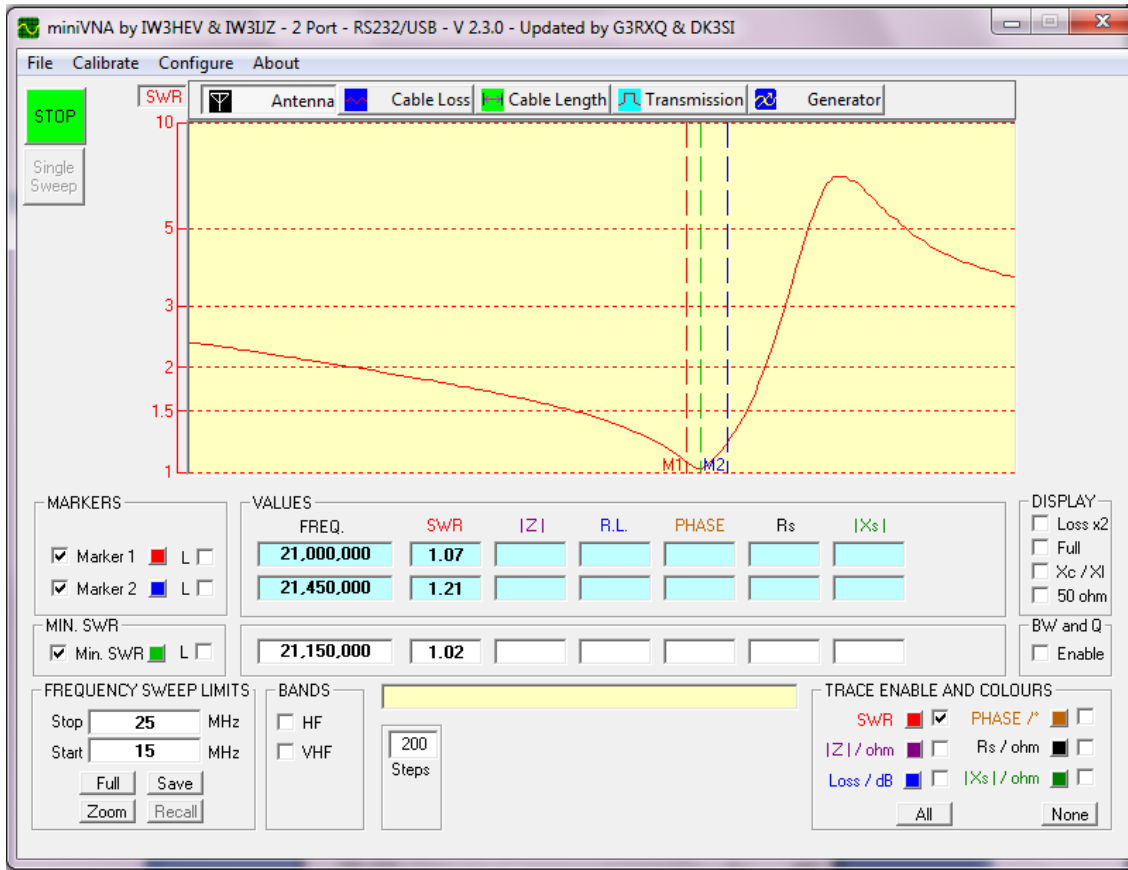
MINIVNA Chart for 15M (21.00, 1.13, 21.300, 1.02, 21.450, 1.10)
