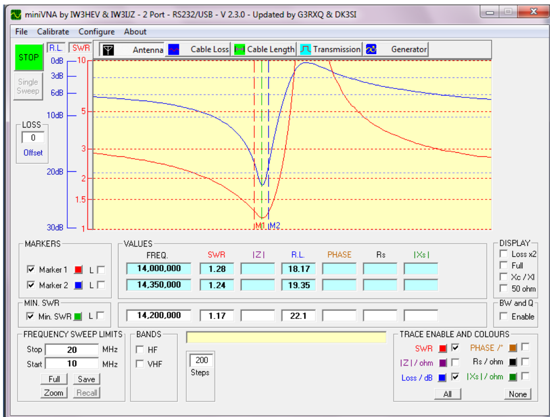
MINIVNA Chart for 20M (14.00, 1.28, 14.200, 1.17 14.350, 1.24)
