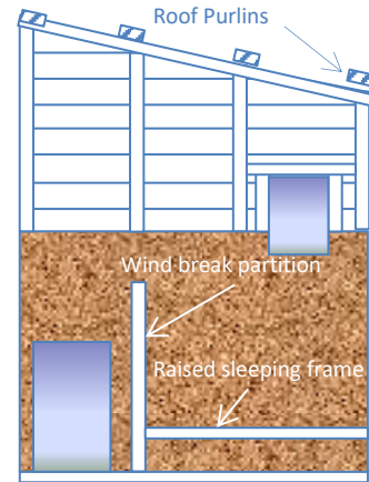
Internal -Pop hole wall, view D
