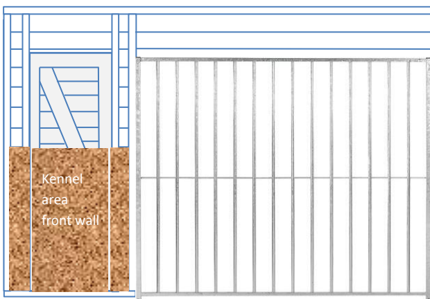
Internal-Front Panel - Inc. kennel, view C
