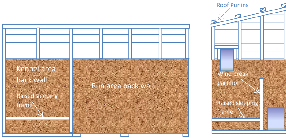
Internal -Pop hole wall, view d
