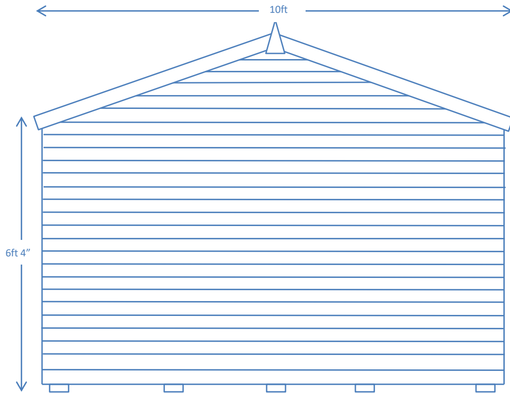
REAR ELEVATION- A
