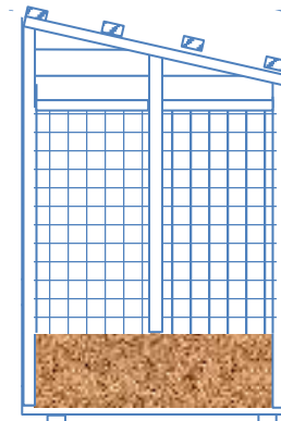
Internal- Run side wall, view b
