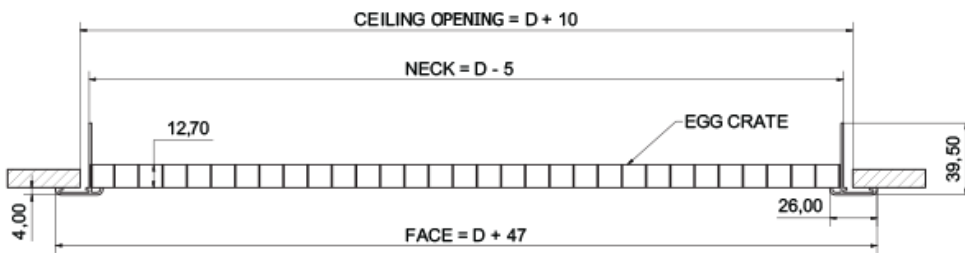
EGG CRATE GRILLE DIMENSIONS
