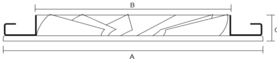
Perforated Face Swirl Diffuser in Tile Grid
