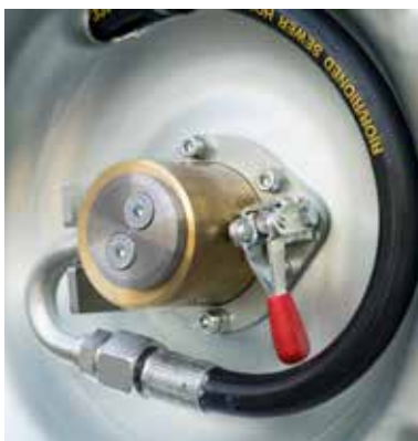
RioFree mechanical freewheel at the hose reel for coiling off without any resistance
