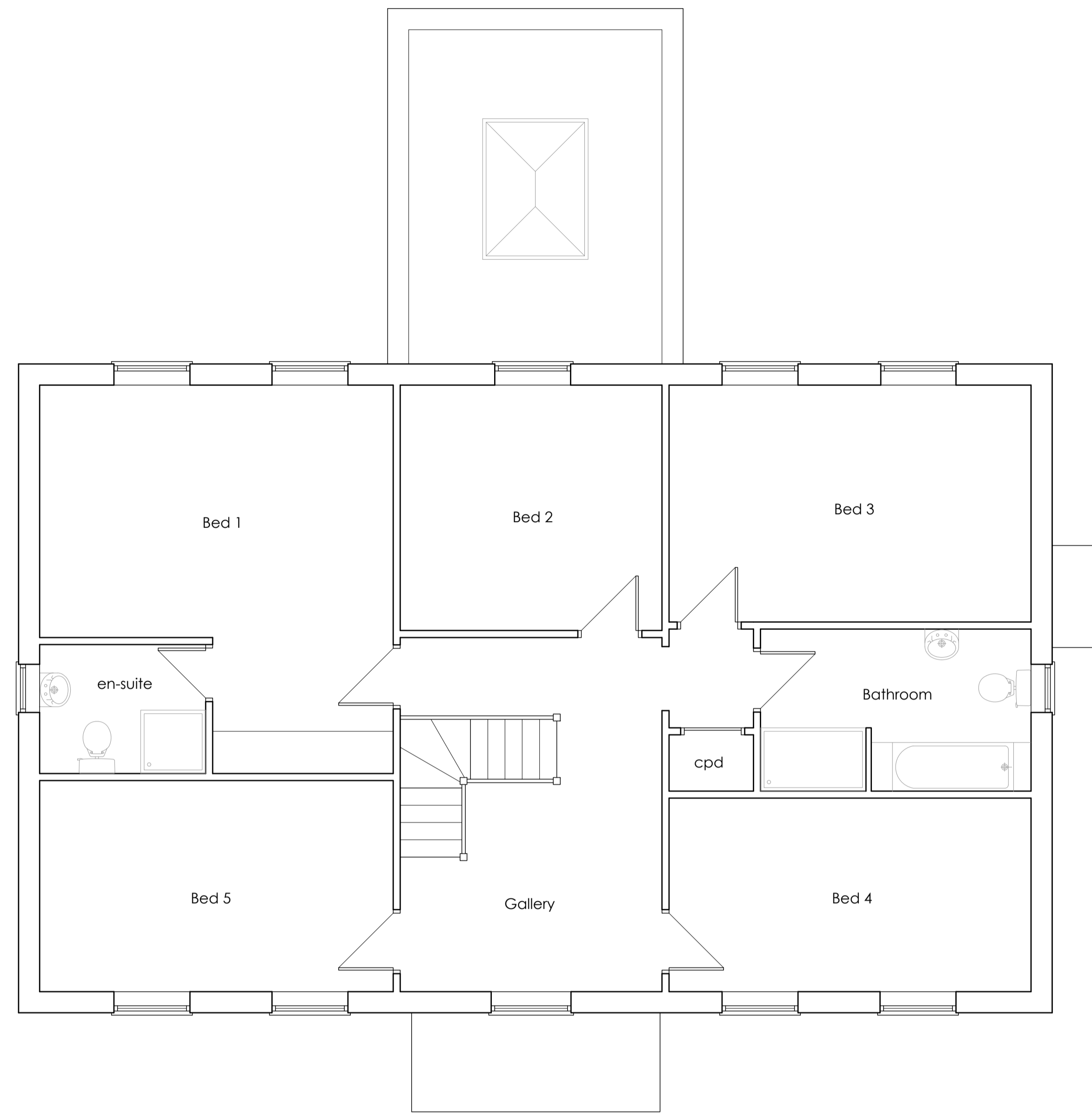
First Floor Layout Plan (1:50)
