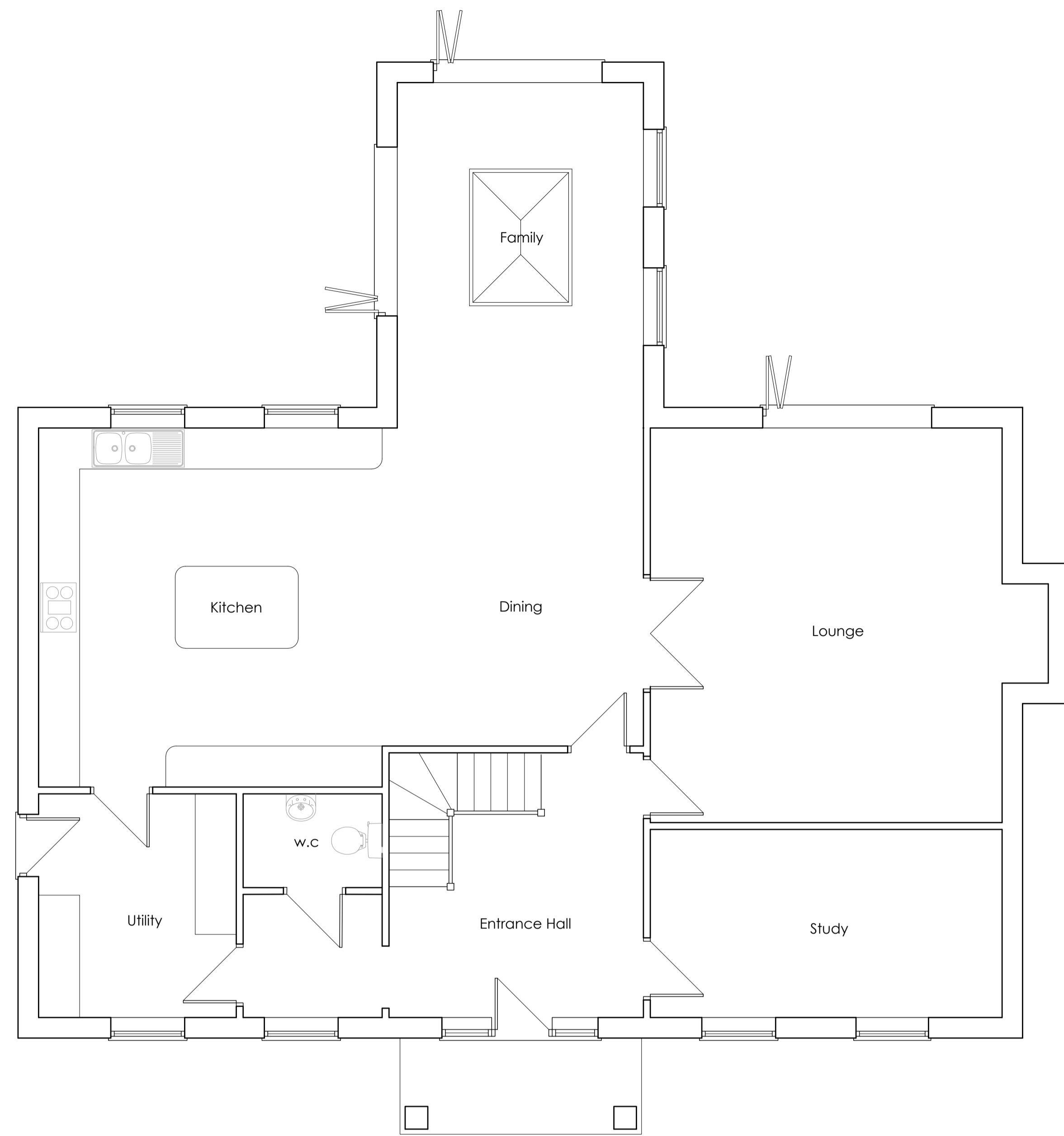
Ground Floor Layout Plan (1:50)
